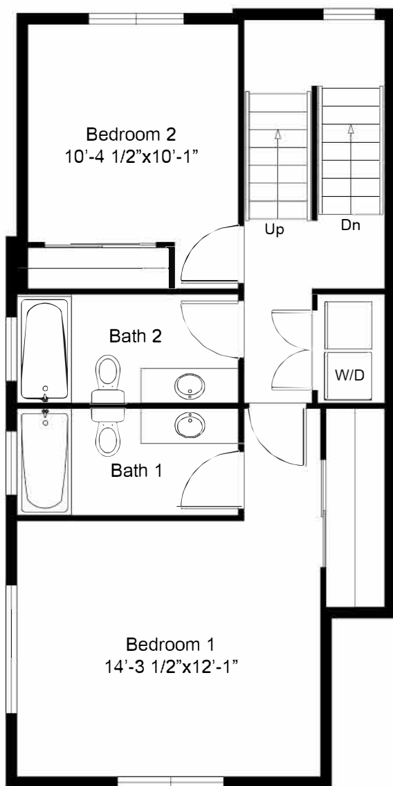
THIRD LEVEL FLOOR PLAN
