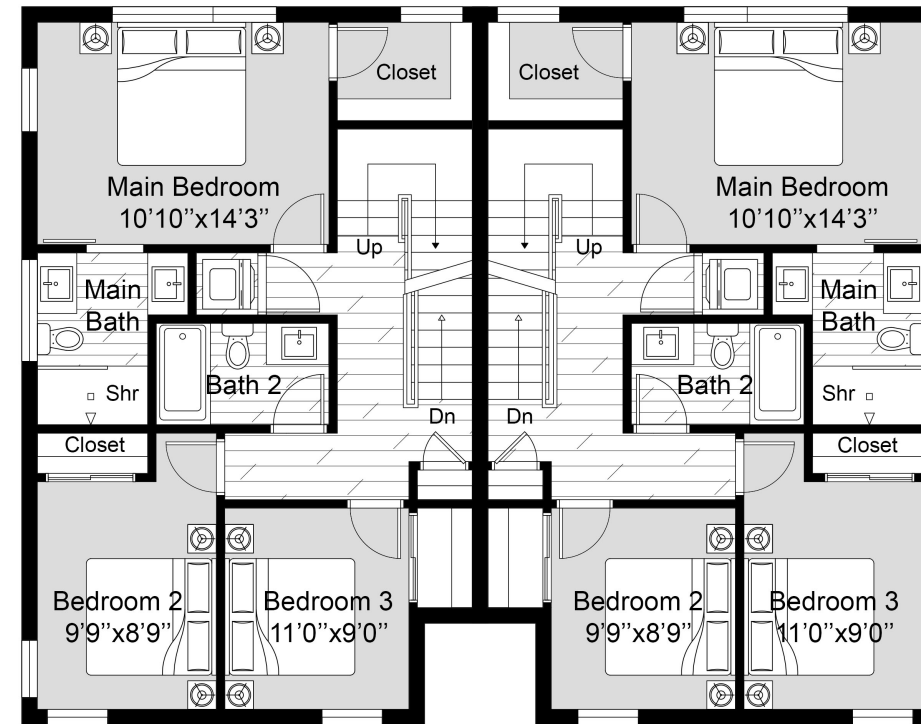
MAIN LEVEL FLOOR PLAN
